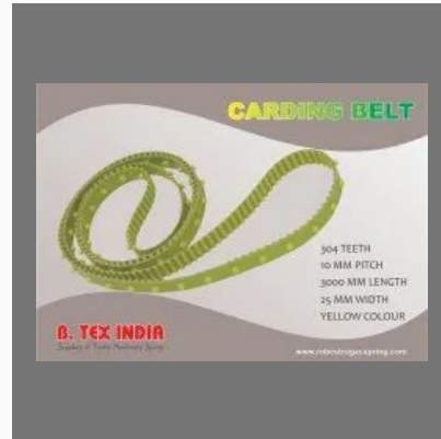
CONVEYOR CARDING BELT AND TRANSPORT BELT
