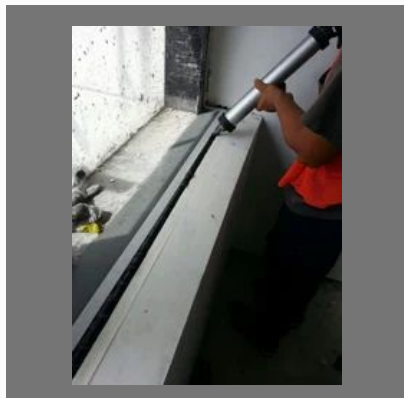
Facade Waterproofing, Silicone Filling & Sealant Application
