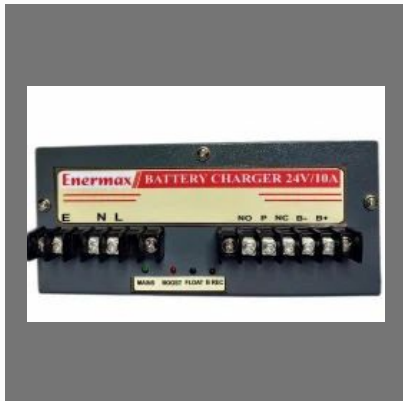
24V/10A Battery Charger For DG Set
