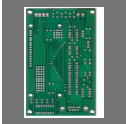
Double Sided Non-PTH
