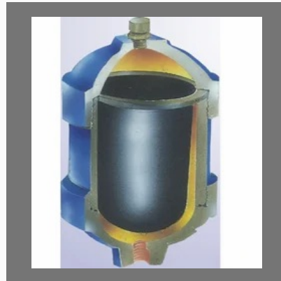
Diaphragm type Accumulators
