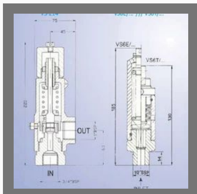
Gas Safety Valves
