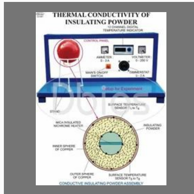
Thermal Conductivity Apparatus Of Insulating Powder
