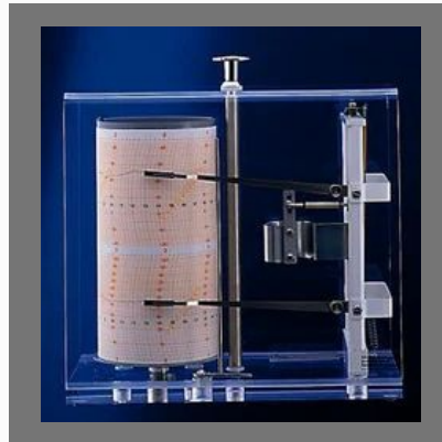
Thermohygrograph
