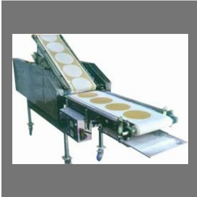
Conveyer Chapathi Machine
