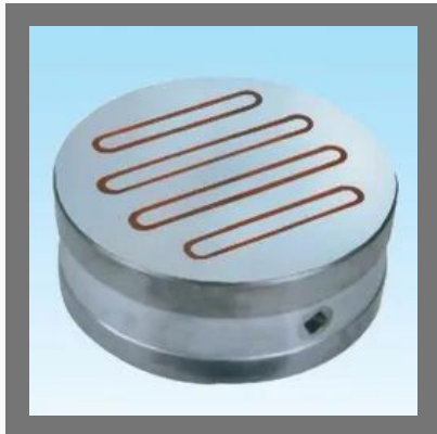
Round Magnetic Chuck
