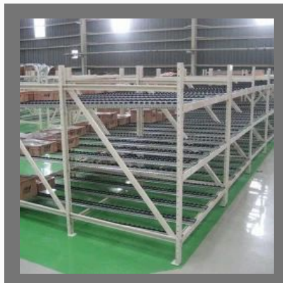
Fifo Flow Rack System
