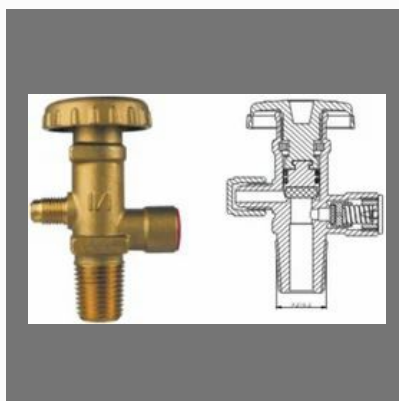
Cylinder Valves
