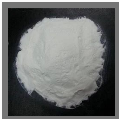
Magnesium Silicate
