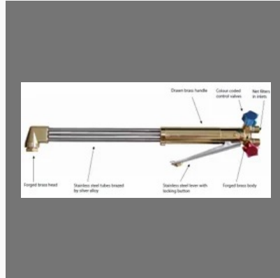
Universal Nm250 Nozzle Mix Heavy Duty Cutting Torch (300 Mm)
