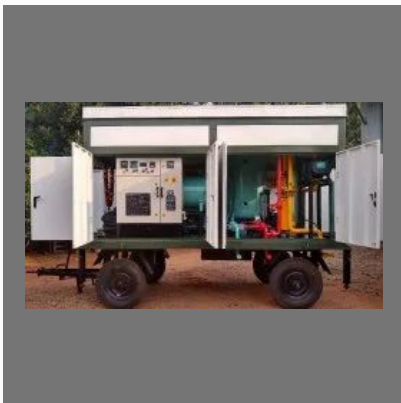
Trolley Mounted Ultra High Vacuum Transformer Oil Filtration Machine
