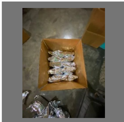
2 3 5 Triiodobenzoic Acid
