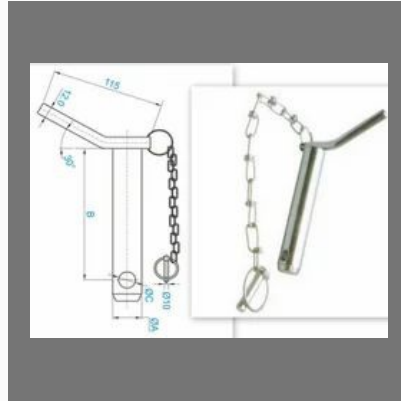
Bent Handle Hitch Pins
