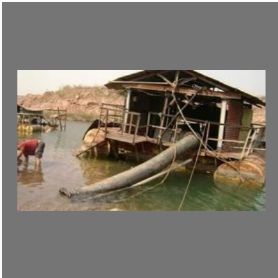
Slurry Hose
