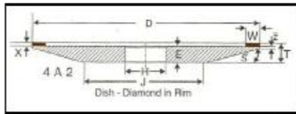
Dish Wheel Type 4A2
