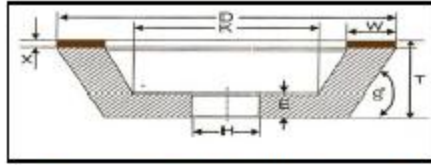
Cup Wheel Type 11A2
