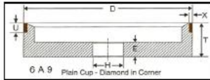
Plain Cup Type 6A9
