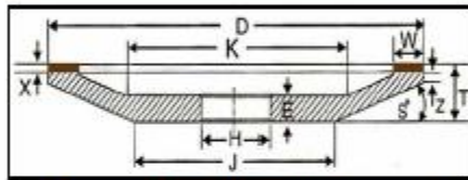
Dish Wheel Type 12A2
