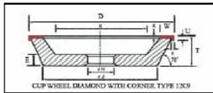
CUP WHEEL DIAMOND WITH CORNER TYPE 12C9
