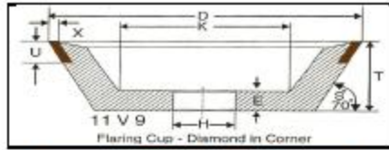
Flaring Cup Type 11V9
