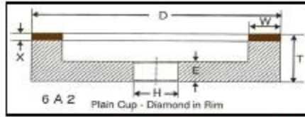
Plain Cup Type 6A2
