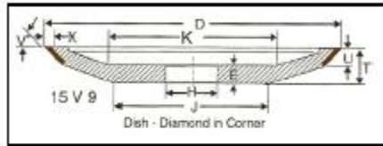
Flared Dish Type 15V9
