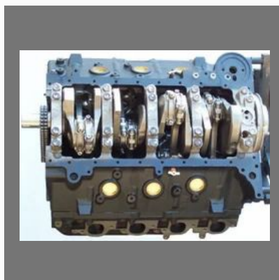
Engine Crankshaft
