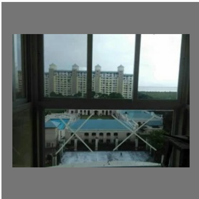
Sliding Window
