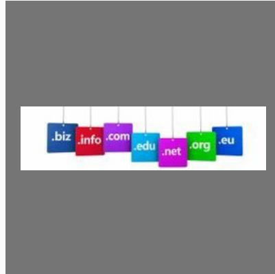
Domain Renewal
