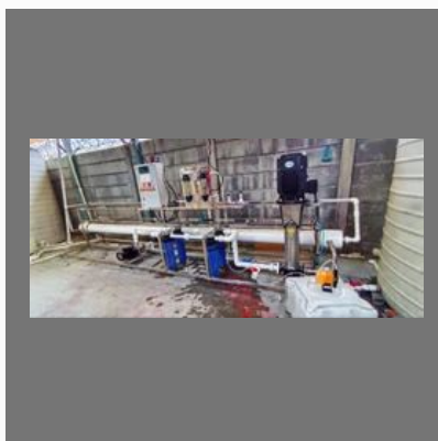
Nanofiltration System
