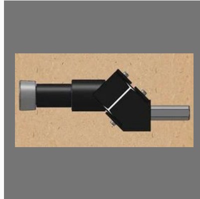
Single Roller Burnishing Blind Bore
