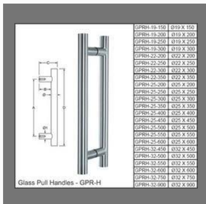
Mortise Handles
