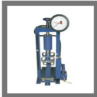
Hand Operated Flexure Testing Machine
