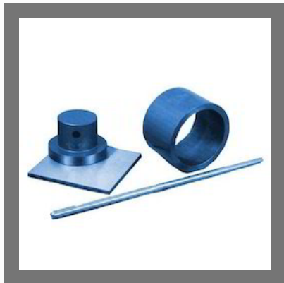
Aggregate Crushing Value Apparatus
