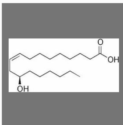
Ricinoleic Acid
