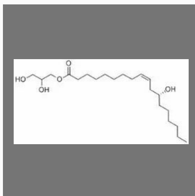
Glyceryl Monoricinoleate
