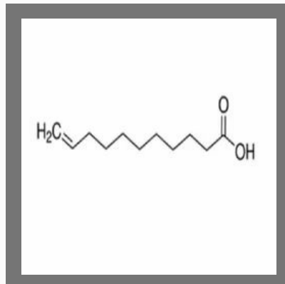
Undecylenic Acid
