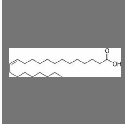
Erucic Acid
