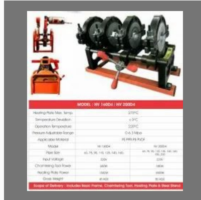
160 mm light manual butt fusion welding machine
