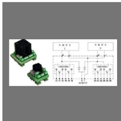
Redundancy Modules
