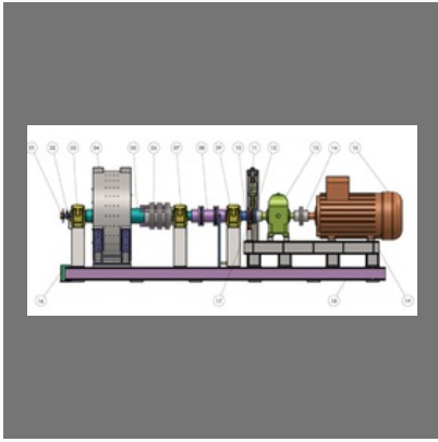
Test Benches And Solutions For Rotary And Static Equipment
