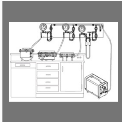
Pressure Plate Apparatus
