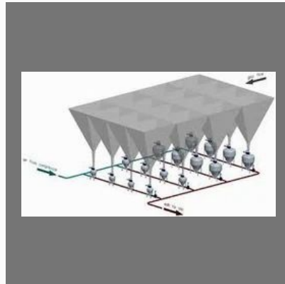
Transporter Vessels
