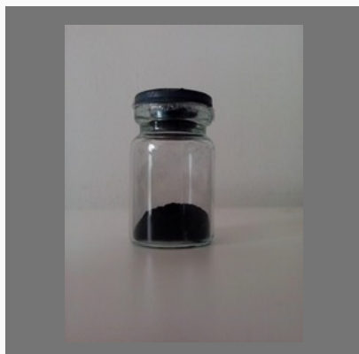
Iridium Calcium Carbonate
