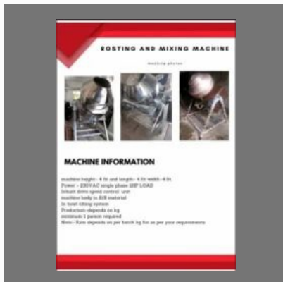
Roasting And Mixing Machine
