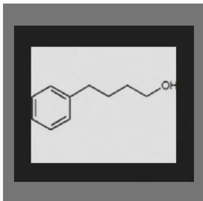
4Phenylbutanol
