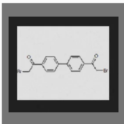
4 4'-2-Chloroacetyl Biphenyl
