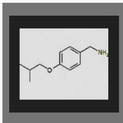
4-Isobutoxybenzylamine
