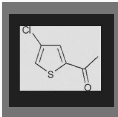
2-Acetyl-4-Chlorothiophene
