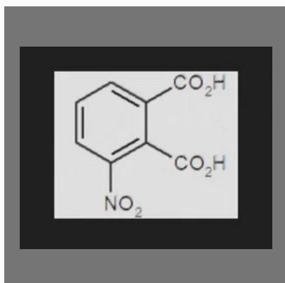
3-Nitrophthalic Acid
