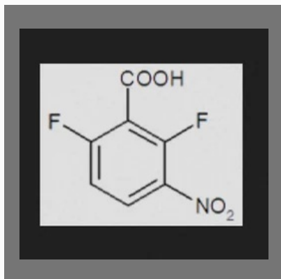
2,6-Difluoro-3-Nitrobenzoic Acid
