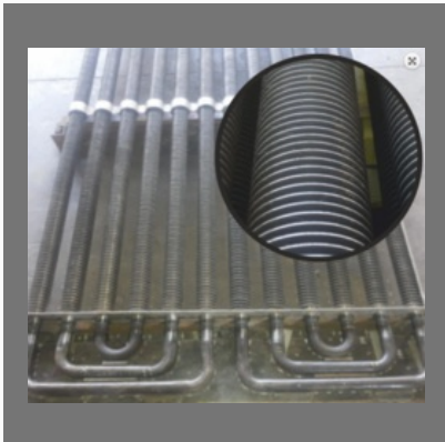
High Frequency Spiral Fin Tube Welded Coils
