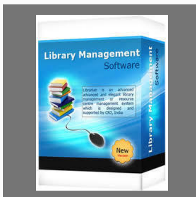
Library Software
