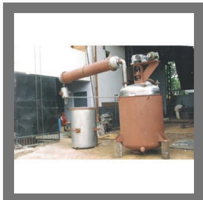
Synthetic Rubber Adhesive Plant
