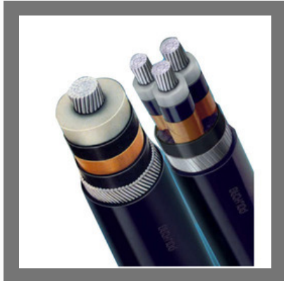
HT XLPE Cable
