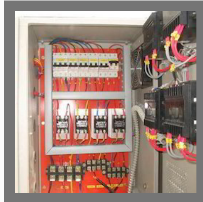
Liquid Automation Control Panel
