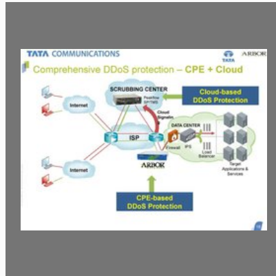
DDoS Services
