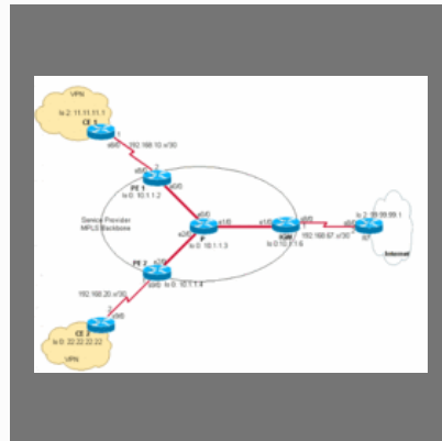
Global MPLS VPN Services
