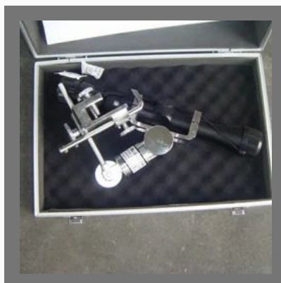
Conductor Sagging Device "Sag-Scope"
