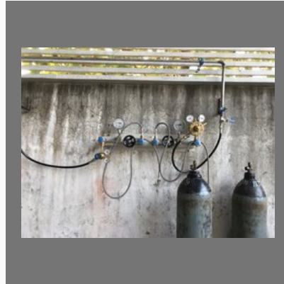
Ss Manifolds
