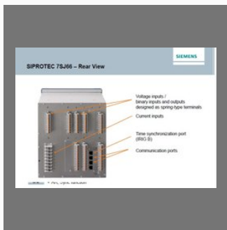
Overcurrent protection SIPROTEC 7SJ66
