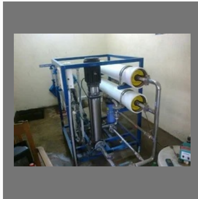
RO Treatment Plant
