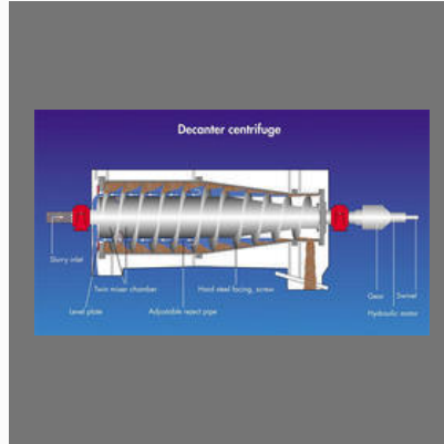
Decanter Centrifuge
