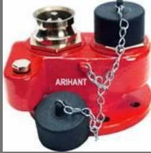
2- Way Breeching Dry Riser Inlet
