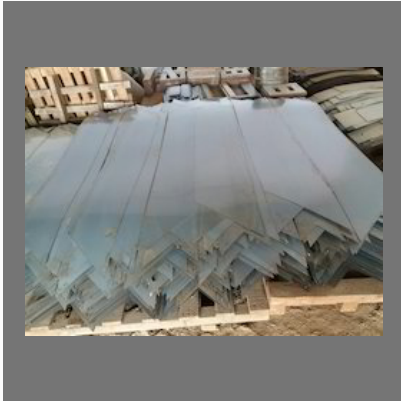
CRGO Lamination Strips
