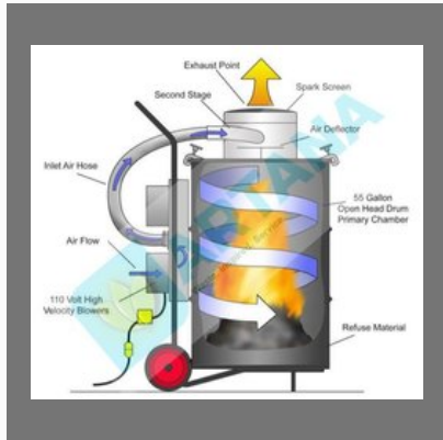
Portable Waste Incinerator
