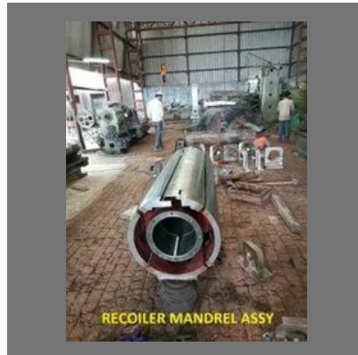
Recoiler Mandrel Assy
