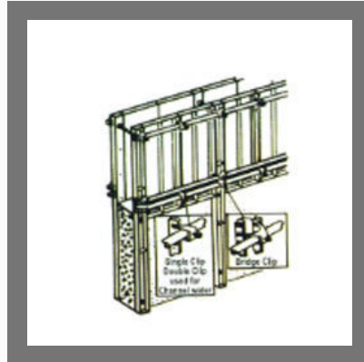
Wall Form Shuttering
