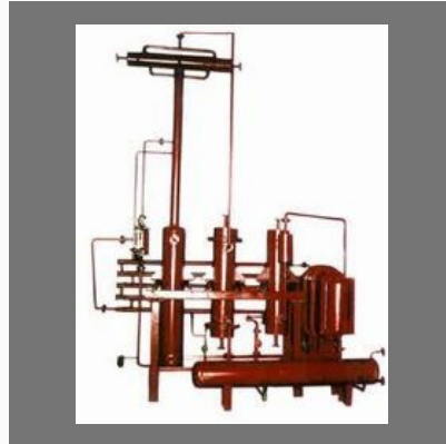
Vapour Absorption Chilling System
